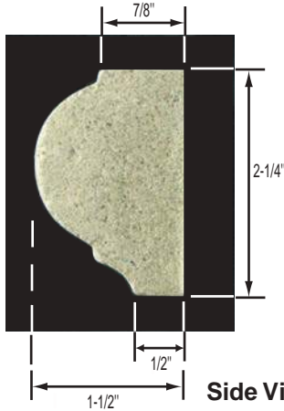
Side View MD-23S
