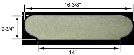
WC-800-14 Side View
