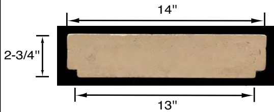
WC-106-13 Side View
